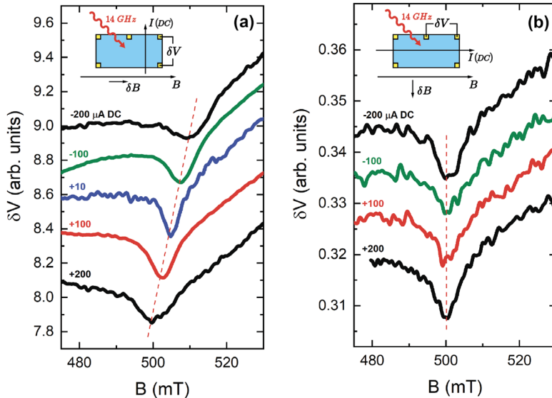
Fig. 1. EPR lines for different orientations of current and measured photovoltage signal. a Effective Bychkov-Rashba magnetic field \delta B is oriented along magnetic field B . A change in current density changes \delta B magnitude, so changes the g -factor. b \delta B is perpendicular to B , so g -factor is constant within the current range under investigation. Resonance frequency is 14 GHz.
