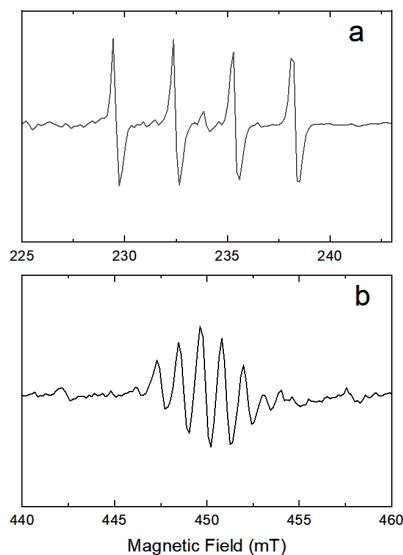
Fig. 1. Spectra of ^{53}\text{Cr}^{3+} ions in \text{Mg}_2\text{SiO}_4 . a single \text{Cr}^{3+} ion; b \text{Cr}^{3+} - \text{Cr}^{3+} dimer associate.
